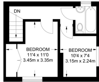
FIRST FLOOR 260 SQ FT / 24.2 SQ M
